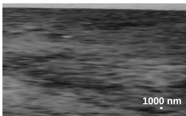
Figure 3. Microstructure of porous polystyrene + amorphous colloid \text{Fe}(\text{OH})_3 , az adsorption centres of over the norm concentration \text{Mn}^{2+} after oxidation of microorganisms \text{Fe}^{2+} \rightarrow \text{Fe}^{3+} after 10 functioning years
